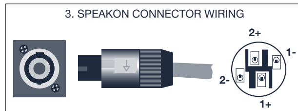
3. Speakon input and output connector wiring.
