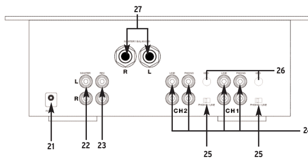
Rear Panel
